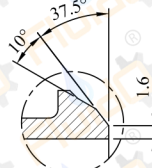
Butt Weld End
