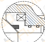
SPRING LOADED DESIGN DETAIL - Y
